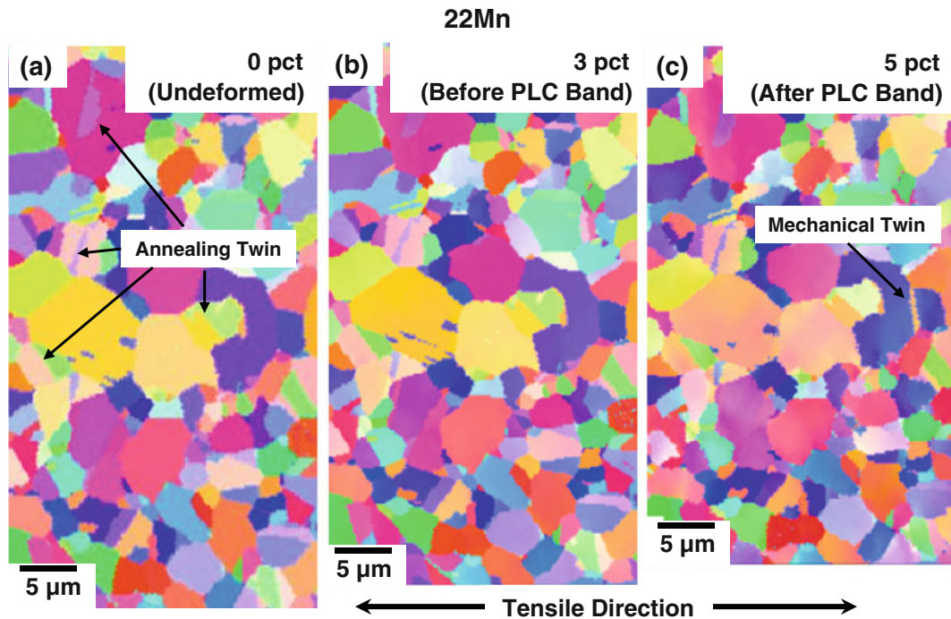
Fig. 9—Inverse pole figure (IPF) color maps of the same observation area after the tensile strain of (a) 0 pct (undeformed), (b) 3 pct (before the formation of PLC deformation band), and (c) 5 pct (after the pass of PLC deformation band) for the 22Mn steel.
