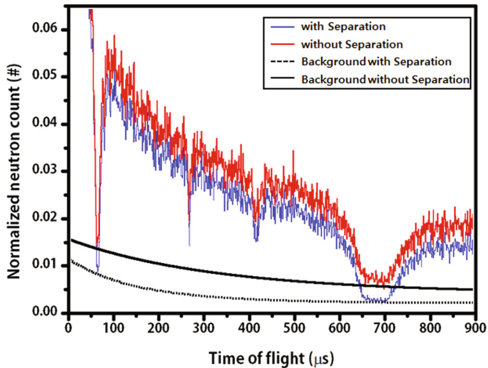
Fig. 5. (Color online) Neutron TOF and background spectra for the notch filter with and without signal and noise separation.
