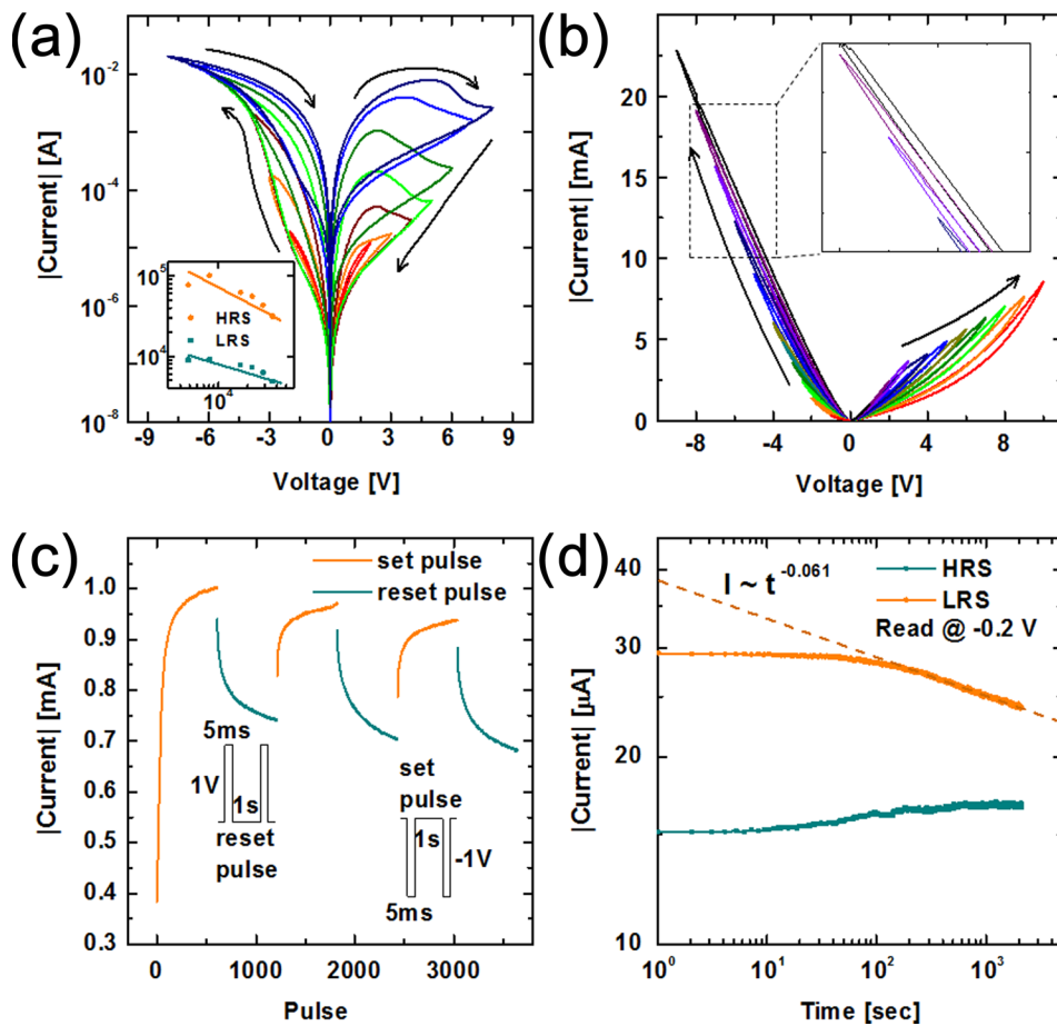
FIG. 2. (a) IV characteristics of the asymmetrical device (H-Pt/NNO/NH-Pt) with gradually increasing the sweeping width of voltages (from -2\text{ V} \leq V \leq 2\text{ V} to -8\text{ V} \leq V \leq 8\text{ V} ). The inset shows resistances at HRS and LRS in devices with various cell areas. (b) IV characteristics with different set and reset voltages applied to H-Pt electrodes repeatedly with sweep widths of -1.0\text{ V} to -9.0\text{ V} in the negative direction and +1.0\text{ V} to +10.0\text{ V} in the positive direction, respectively. The inset shows the enlarged plot in the range of the negative bias of the IV curves. (c) Conductance modulation by iterative small voltage pulses with 600 potentiating (or set) pulse sequences first and then the successive 600 depressing (or reset) pulse sequences. The voltage level and duration in pulses were set to \pm 1\text{ V} and 5 ms, respectively, with a 1 s interval. (d) Retention test of our protonic memory resistors. The current was measured at -0.2\text{ V} for HRS and LRS.
